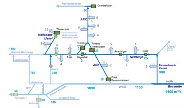
Figure 4.2: Water distribution of the Rhine branches with a Rhine discharge of 1400 m³/s (Spijker & van den Brink, 2013)
