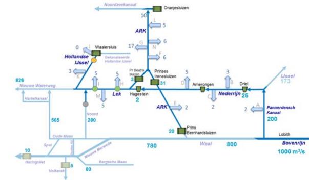
Figure 4.3: Water distribution of the Rhine branches with a Rhine discharge of 1000 m³/s (Spijker & van den Brink, 2013)
